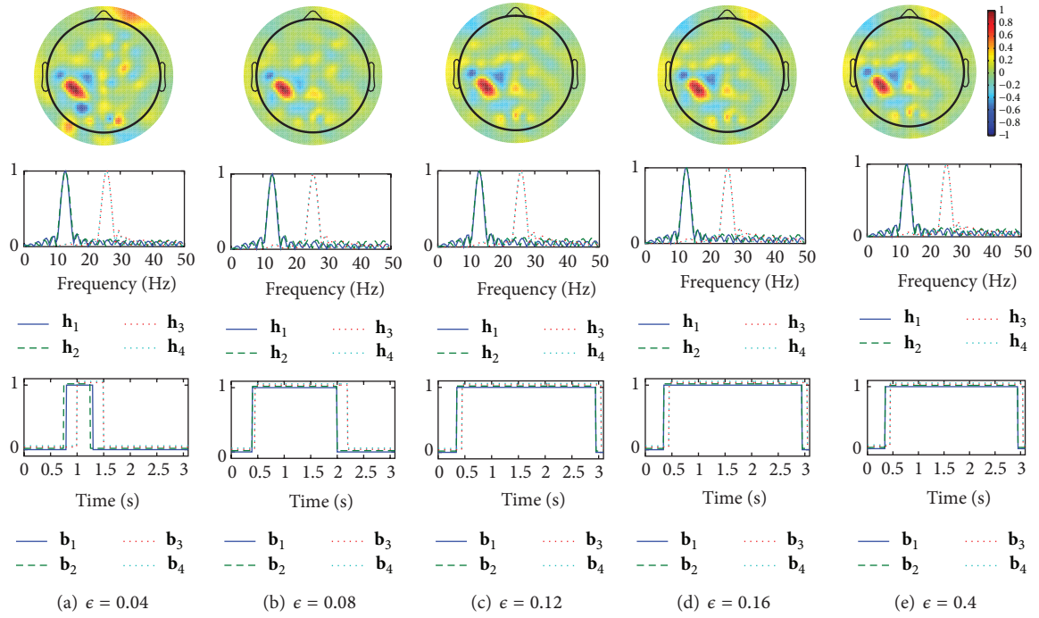
FIGURE 7: Examples of spatio-time-frequency patterns as the spatial weights, \hat{\mathbf{w}}_1^{(1)} (top), the amplitude response of the filter, \mathbf{h}_1, \dots, \mathbf{h}_4 (center), and the time windows, \mathbf{b}_1, \dots, \mathbf{b}_4 (bottom), designed by the CSTFP method with various \epsilon in the result of subject aa . The vertical axis represents normalized amplitude.
