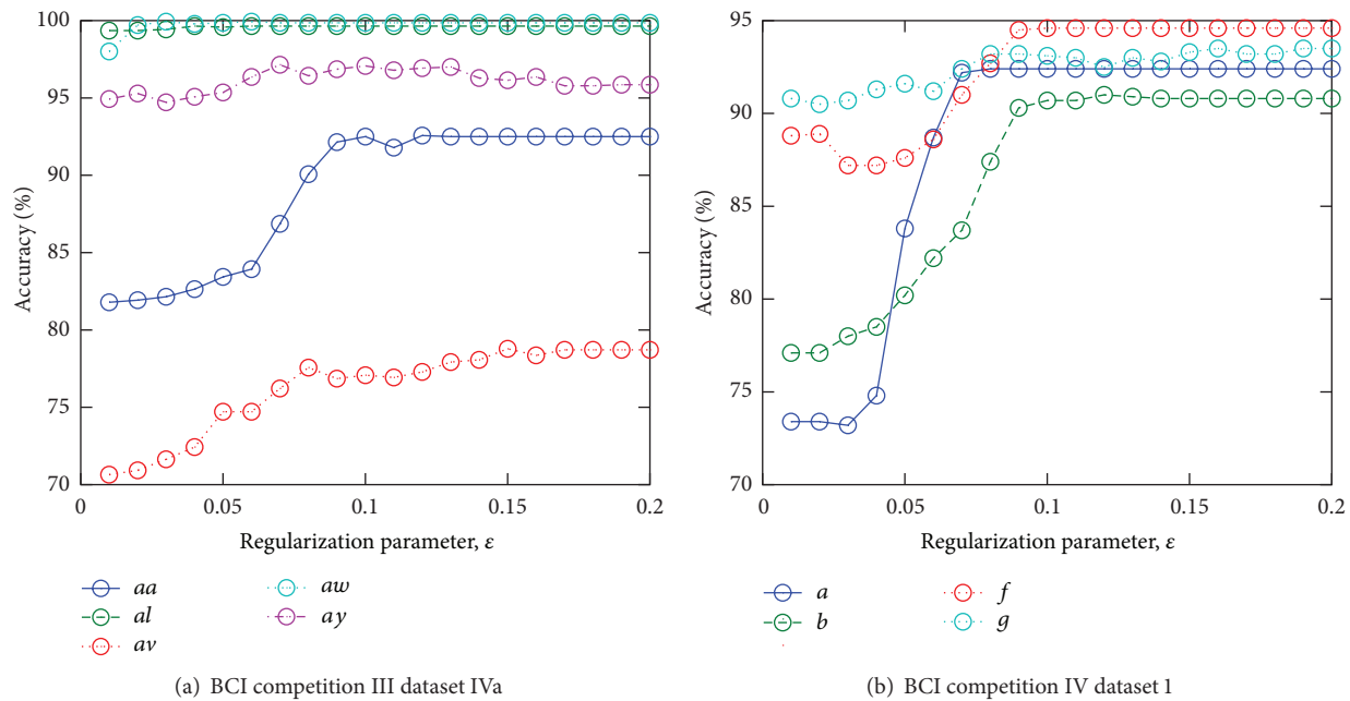
FIGURE 6: The variation of the accuracy rates by various regularization parameters, \epsilon .
