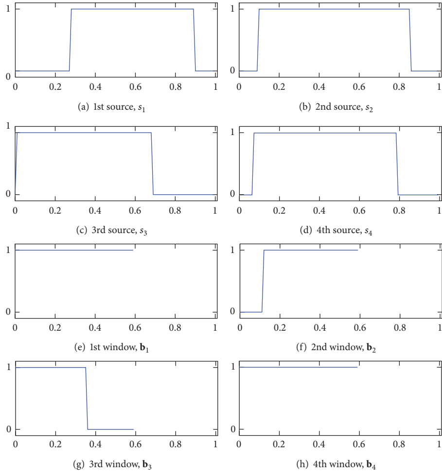
FIGURE 3: Time patterns as the time windows of the source signals ((a)–(d)) and the designed time windows ((e)–(h)). The horizontal axis represents time and its unit is the second.
