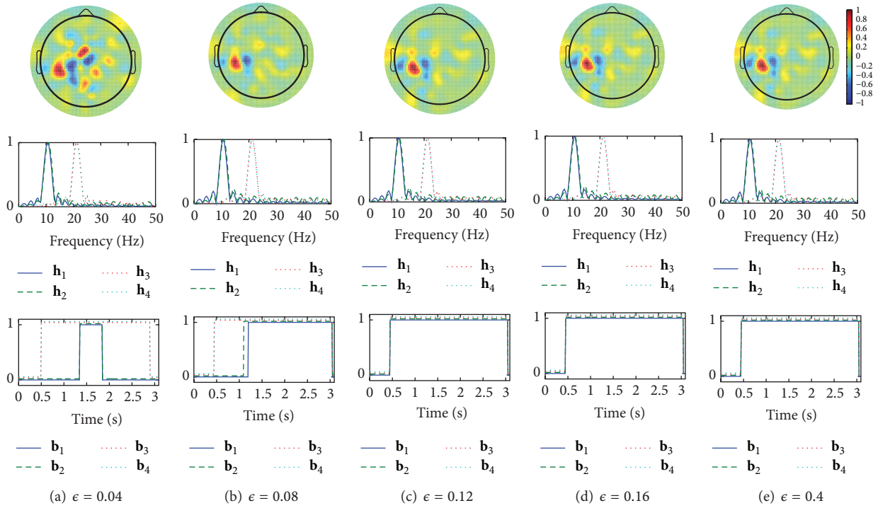
FIGURE 8: Examples of spatio-time-frequency patterns as the spatial weights, \hat{\mathbf{w}}_1^{(1)} (top), the amplitude response of the filter, \mathbf{h}_1, \dots, \mathbf{h}_4 (center), and the time windows, \mathbf{b}_1, \dots, \mathbf{b}_4 (bottom), designed by the CSTFP method with various \epsilon in the result of subject av . The vertical axis represents normalized amplitude.
