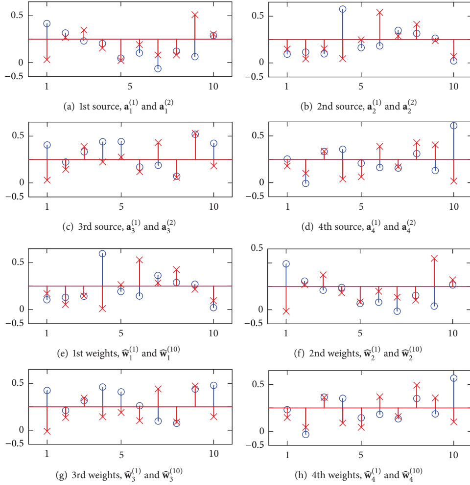
FIGURE 4: Spatial patterns as the spatial amplitudes of the source signals ((a)–(d)) and the designed spatial weights ((e)–(h)). The amplitudes plotted by circles are \mathbf{a}_i^{(1)} and the amplitudes plotted by cross are \mathbf{a}_i^{(2)} for i = 1, \dots, 4 . The weights plotted by circles are \mathbf{w}_i^{(1)} and the weights plotted by cross are \mathbf{w}_i^{(10)} for i = 1, \dots, 4 . The horizontal axis represents the channel number.
