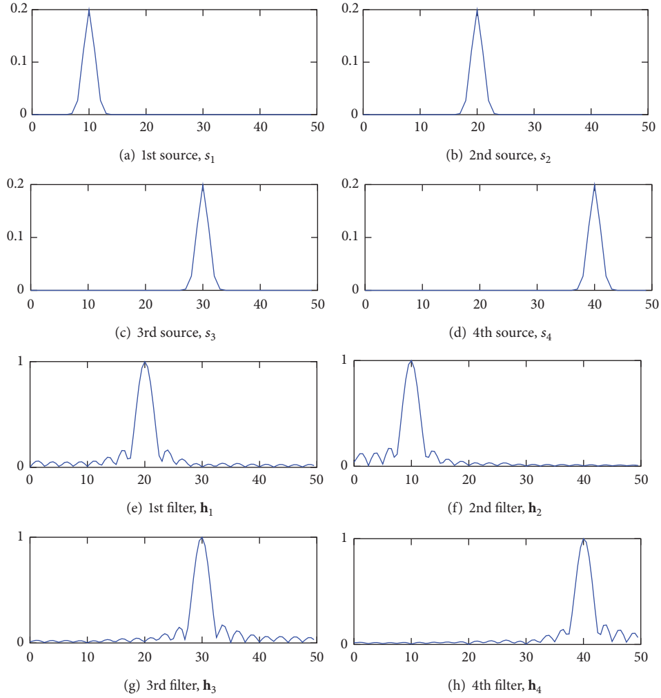
FIGURE 2: Frequency patterns of the spectra of the source signals ((a)–(d)) and the amplitude characteristics of the designed frequency patterns ((e)–(h)). The horizontal axis represents frequency and its unit is Hz.
