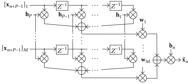
FIGURE 1: The filtering of an observed signal by a temporal filter, \mathbf{h} , spatial weights, \mathbf{w} , and a time window, \mathbf{b} . Z^{-n} is an operator of n samples delay.
